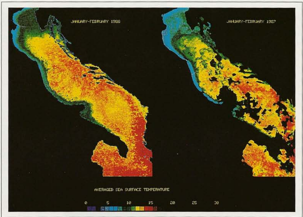
Fig. 12.6. Two-month composite of NOAA AVHRR data for January—February for the years 1986 and 1987. At this time, the composite of mean radiation temperatures indicate that the Po waters are shown to flow in a narrow stream southward along the Italian coast. (From Marullo and La Violette, 1991.)
