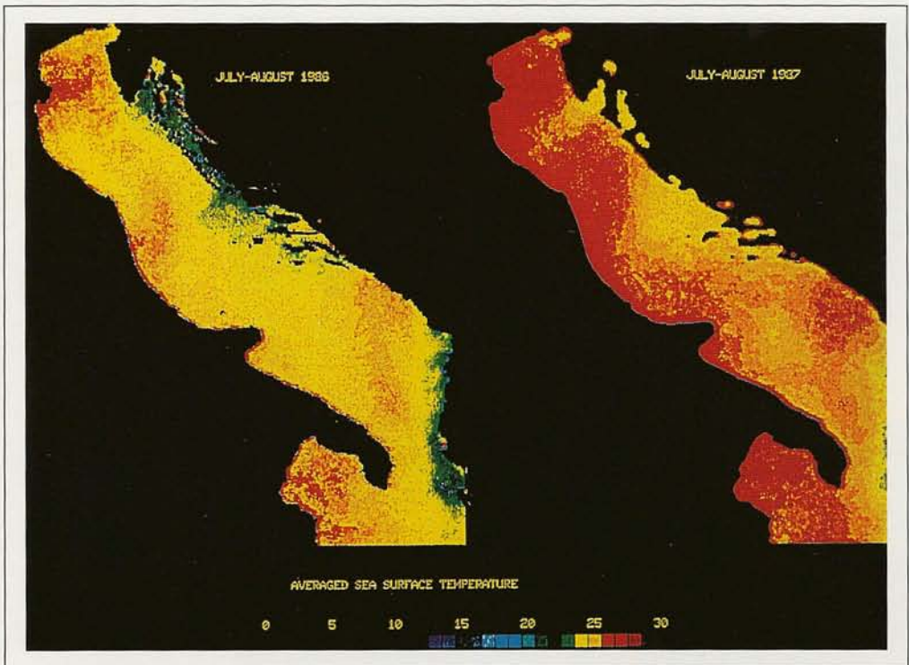
Fig. 12.7. Two-month composite of NOAA AVHRR data for July—August for the years 1986 and 1987. The composite of mean radiation temperatures indicate that the Po River outflow is diverted into the northern basin and retained in that area during the summer. (From Marullo and La Violette, 1991.)
