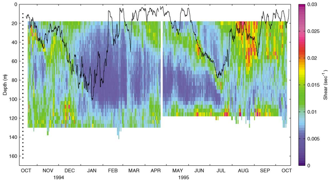
Fig. 9. The daily average vertical shear of the horizontal velocity, as measured by the ADCP on SIO-S. Black dots at left indicate the depths of the measurement bins. The daily mean mixed layer depth from WHOI is superimposed.
