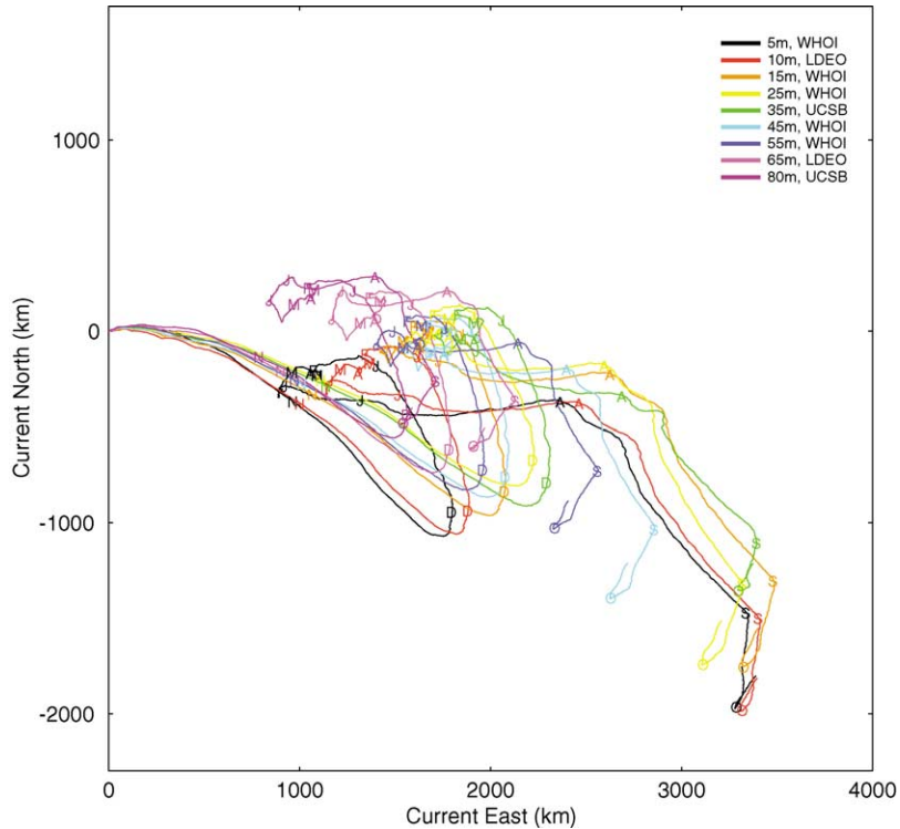
Fig. 8. Progressive vector diagrams (time-integrated velocity) from the current meters on WHOI. All are given a common start, and the first days of each month, starting with November 1994, are marked.
