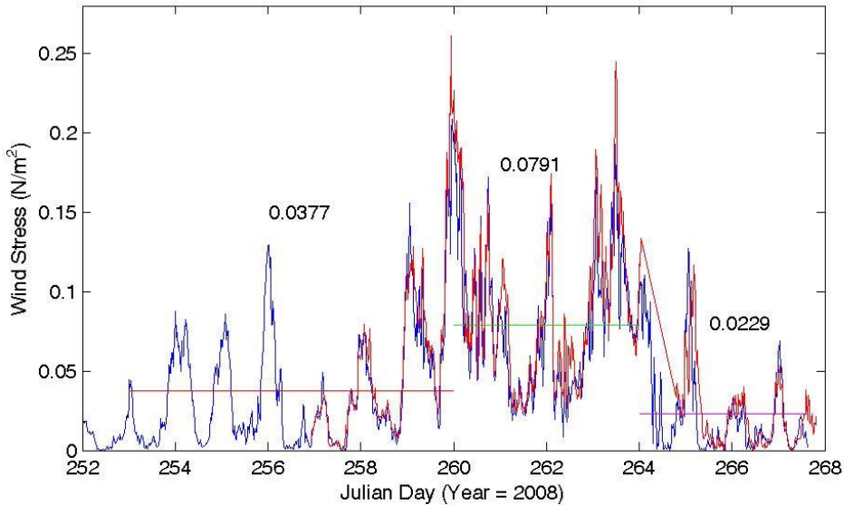
Wind Stress From KM (Blue) and FLIP (red), mean values are calculated from KM data
