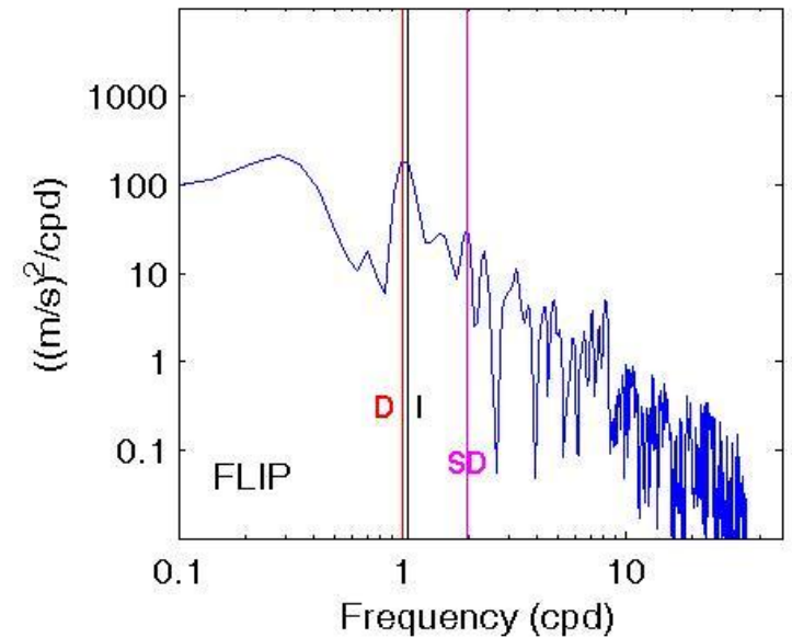
Wind Speed Spectra (FLIP), Sept. 13-23, 2008
