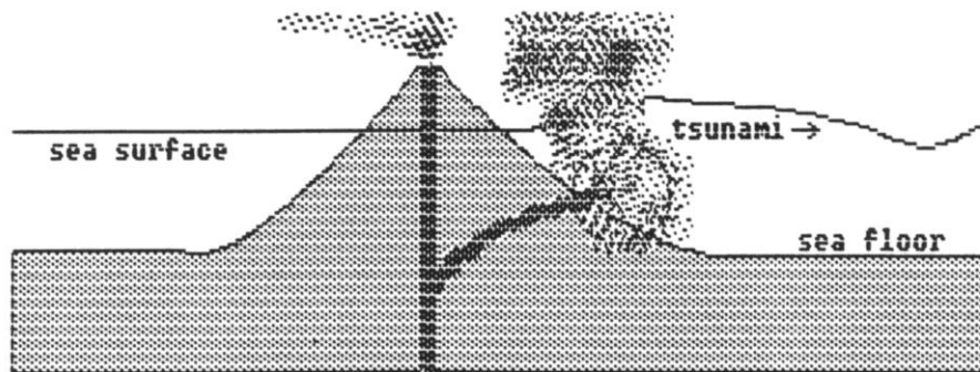
Figure 2.4 Graphic representation of a tsunami produced by submarine volcanic explosion.
