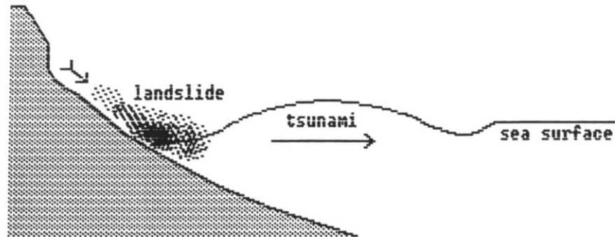
Figure 2.3 Graphic representation of a tsunami generated by landslide originating above sea level.
