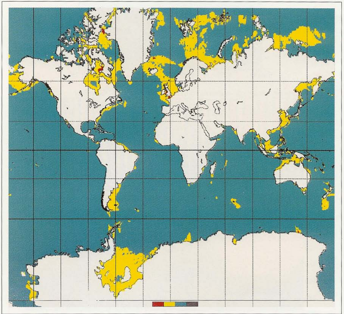
Fig. 5.3. Global distribution of dissipation from the model of Le Provost et al. (1994). Areas in yellow have dissipation > 10^{-4} \text{ W m}^{-2} ; in red, > 10^{-1} \text{ W m}^{-2} . (Courtesy of F. Lyard, personal communication.)
