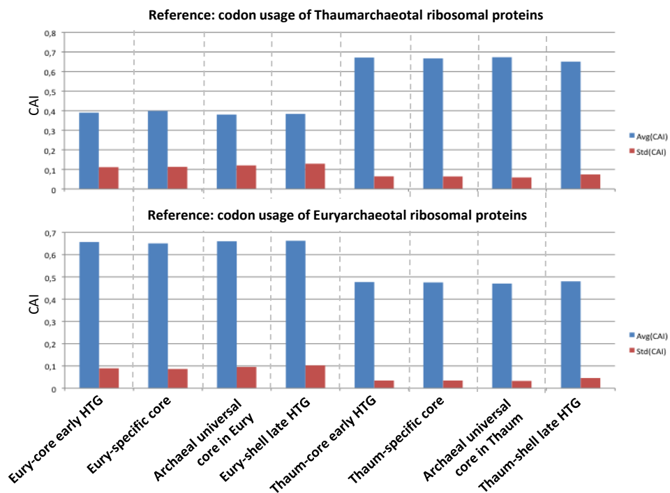
Fig. S7. Codon adaptation index (CAI) of different gene classes in deep-sea Thaumarchaeota and GII/III-Euryarchaeota as referred to the codon usage of thaumarchaeotal (Thaum) or GII/III-euryarchaeotal (Eury) ribosomal genes. Avg, average value; Std, standard deviation. HTG, horizontally transferred genes.
