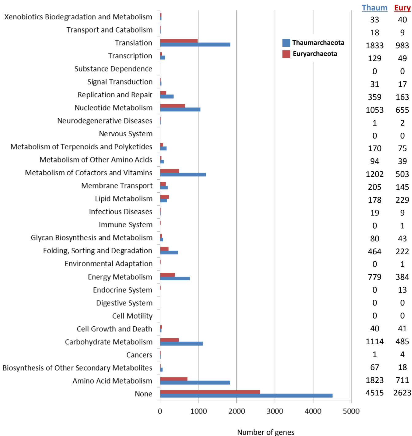
Fig. S4. Comparative distribution of genes in KEGG classes for the Thaumarchaeota (blue) and the Group II/III Euryarchaeota (red) in deep-Mediterranean archaeal fosmid metagenome sequence. Total gene numbers are given on the right.
