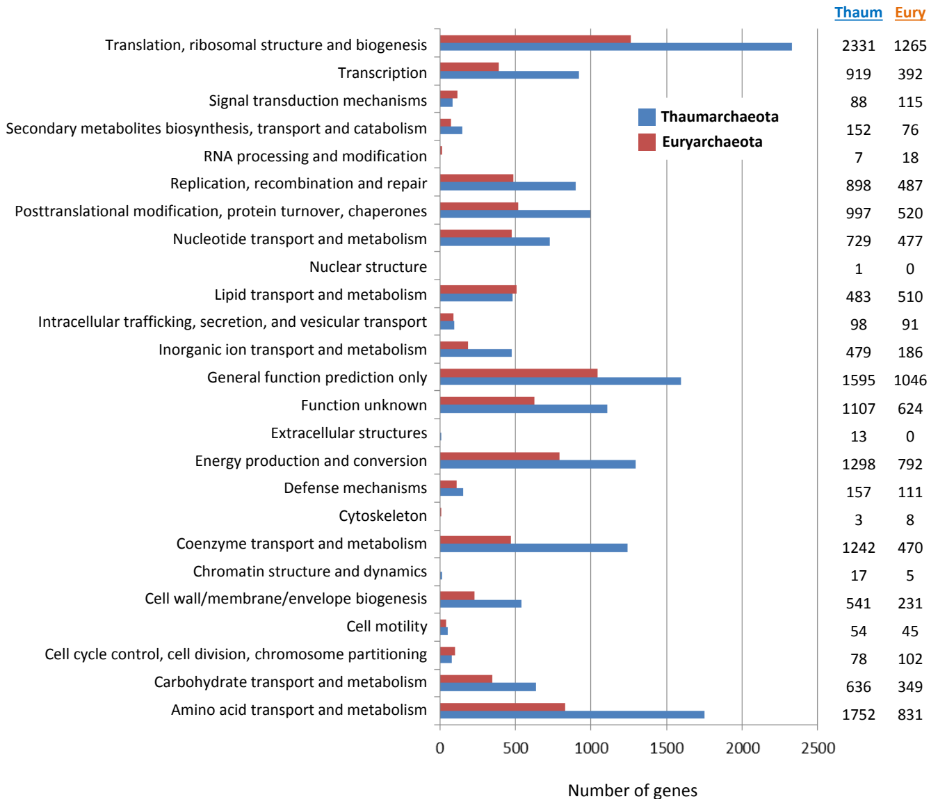
Fig. S3. Comparative distribution of genes in COG categories for the Thaumarchaeota (blue) and the Group II/III Euryarchaeota (red) in deep-Mediterranean archaeal fosmid metagenome sequence. Total gene counts are given on the right.
