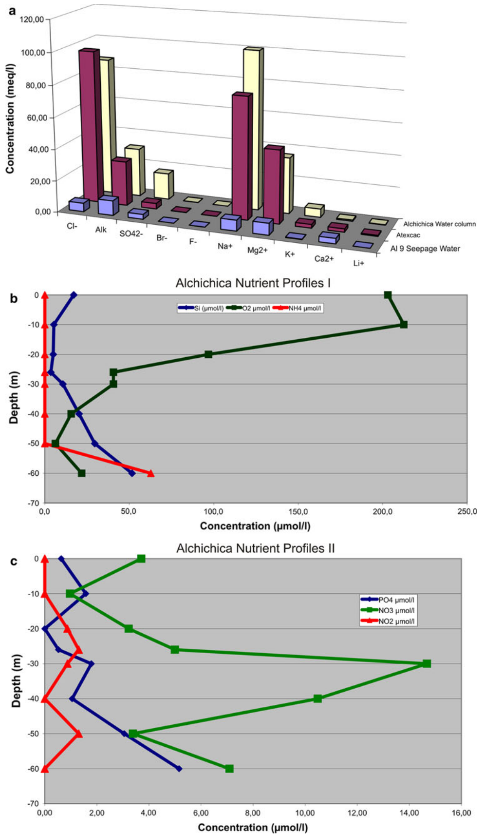
Fig. 4 a Comparison of the major ions of the three water bodies (mean of eight Alchichica water column samples), Alchichica seepage water, and the neighbor crater lake Atexcac (see Fig. 1a). b , c Vertical profiles of oxygen, silicon, and ammonium concentrations ( b ), and of nitrite, nitrate and phosphate ( c )
