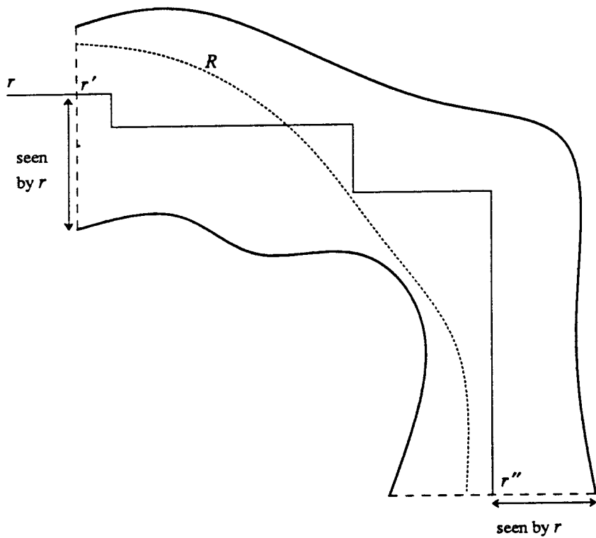
Figure 9: Proof of Lemma 11
