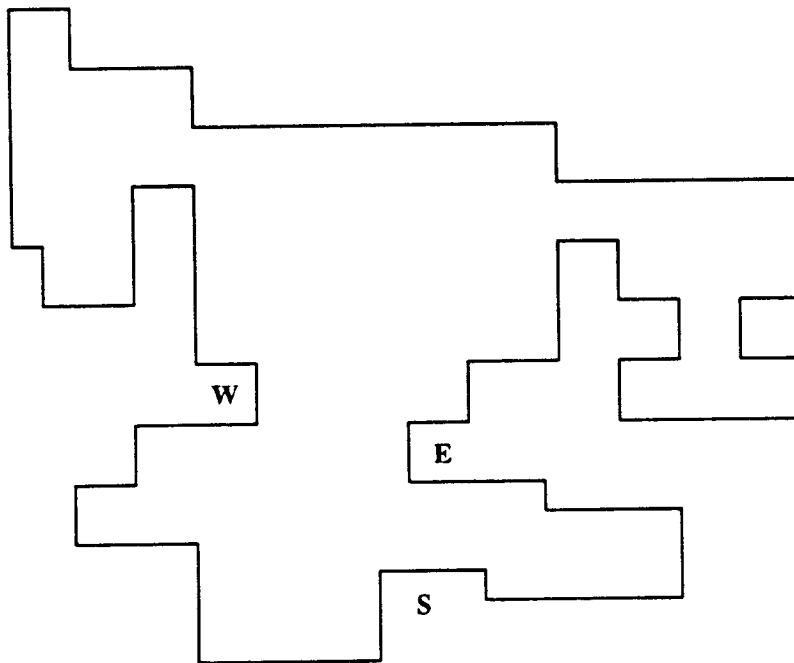
Figure 2: A Polygon with only 3 dent orientations
