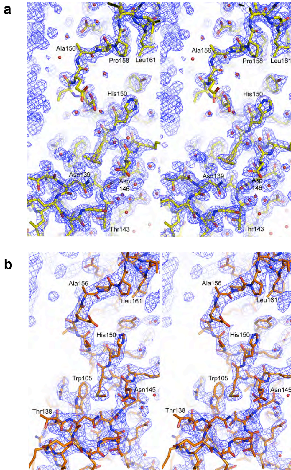
Supplementary Figure 1 Representative electron density ( 2F_o - F_c , 1\sigma x RMSD) surrounding the flap region in the IST1 NTD crystal structures.
