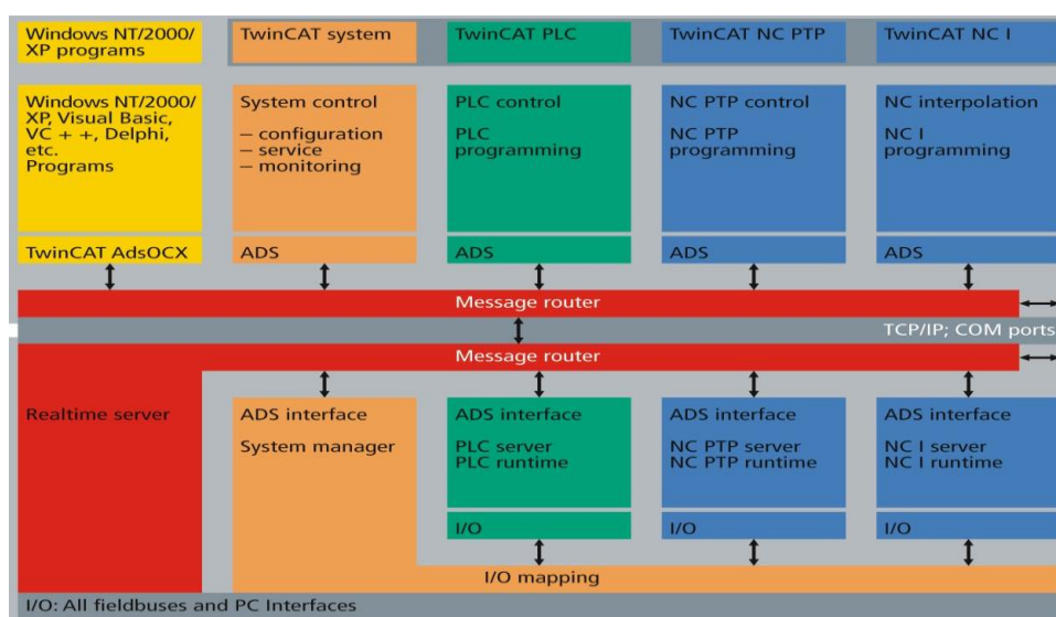
Figure 2. TWINCAT System Frame Basis ADS
