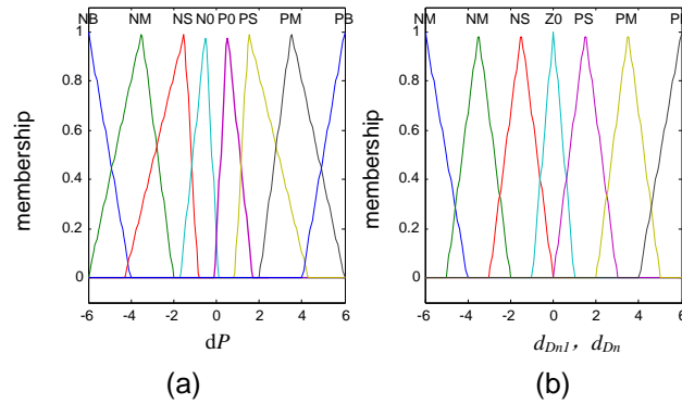
Figure 4. Membership Functions of dP (a), d_{Dn1} and d_{Dn} (b)
