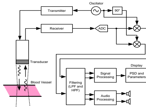
Figure 1. Main Structure of TCD Ultrasound System
