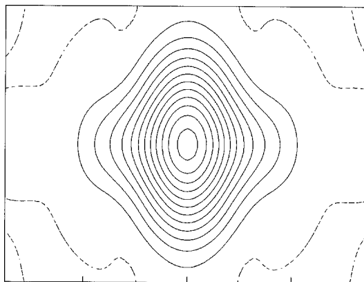
FIG. 3. A difference-Fourier section through the A(2/m) site parallel to (01) and calculated with the A-group cations removed from the structure model; the contour interval is 1 \text{ e}/\text{\AA}^3 , and the dashed line is the zero contour.
