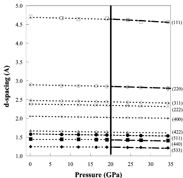
Figure 2. Pressure dependences of d spacings calculated from the observed diffraction peaks of nanocrystalline spinel \text{Ge}_3\text{N}_4 .
