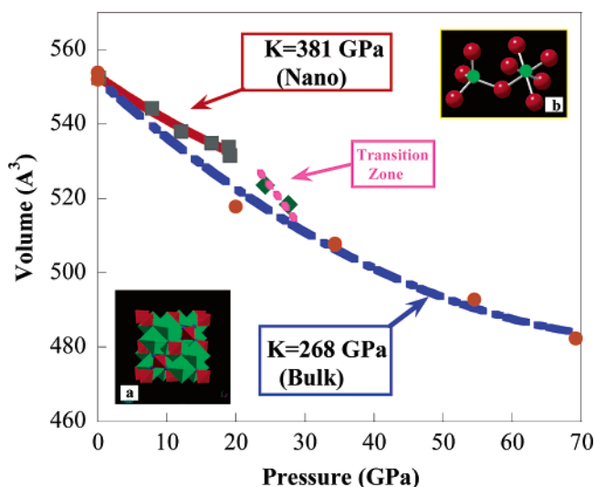
Figure 3. The EOS curves fitted from the volumetric data obtained at pressures below and above 20 GPa. Note: two data points for bulk \text{Ge}_3\text{N}_4 at 0 and 20 GPa are from refs 12 and 13. Inset a shows the structure of spinel \text{Ge}_3\text{N}_4 with octahedron (green) and tetrahedron (red); inset b shows details of octahedron and tetrahedron of spinel: green balls represent Ge atoms and red balls represent N atoms.
