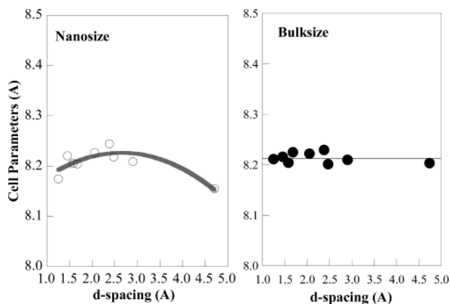
Figure 1. Relationship between d spacing and cell parameter ( a ) of spinel \text{Ge}_3\text{N}_4 at ambient conditions: (a) nanocrystalline; (b) bulk \text{Ge}_3\text{N}_4 .
