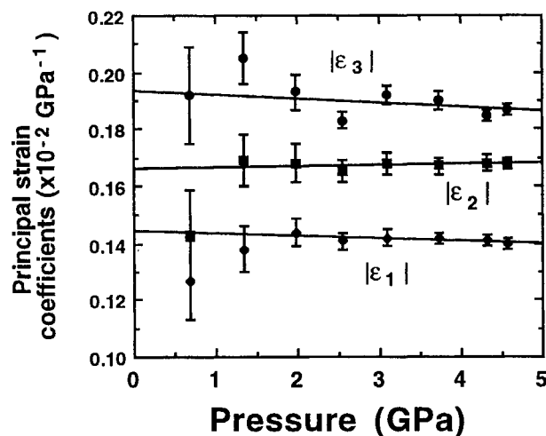
FIGURE 2. The magnitudes of the principal unit-strain coefficients as a function of pressure. The solid lines represent the best linear fits to the data.
