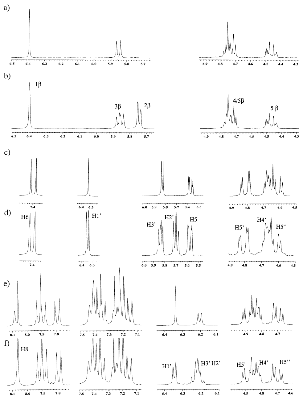
Fig. 1. Expanded regions of the 270-MHz 1D - ^1H NMR spectra of 1-O-acetyl-2,3,5-tris-O-(4-toluoyl)- \beta -D-[2- ^2H_1 ]ribose ( 11 \beta ) (a) and its natural-abundance counterpart (b), 2',3',5'-tris-O-(4-toluoyl)-[2- ^2H_1 ]uridine ( 12a ) (c) and its natural-abundance counterpart (d), N 2 -acetyl-O 6 -(diphenylcarbamoyl)-2',3',5'-tris-O-(4-toluoyl)[2- ^2H_1 ]guanosine ( 12b ) (e) and its natural-abundance counterpart (f)
