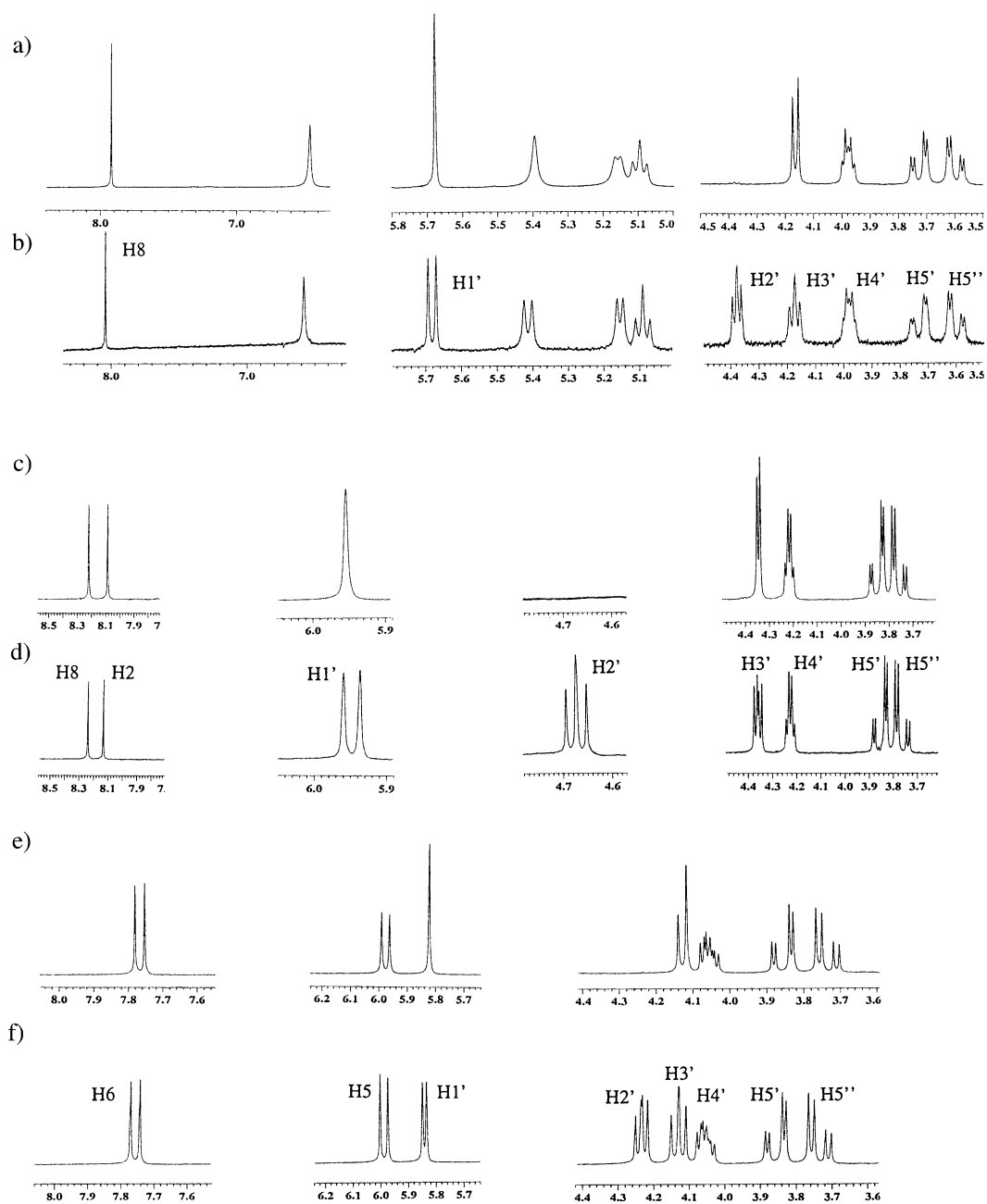
Fig. 3. Expanded regions of the 270-MHz 1D - ^1H NMR spectra of [2\text{'-}^2H_1] guanosine ( 13b ) (a) and its natural-abundance counterpart (b), [2\text{'-}^2H_1] adenosine ( 13c ) (c) and its natural-abundance counterpart (d), [2\text{'-}^2H_1] cytidine ( 13d ) (e) and its natural-abundance counterpart (f)
