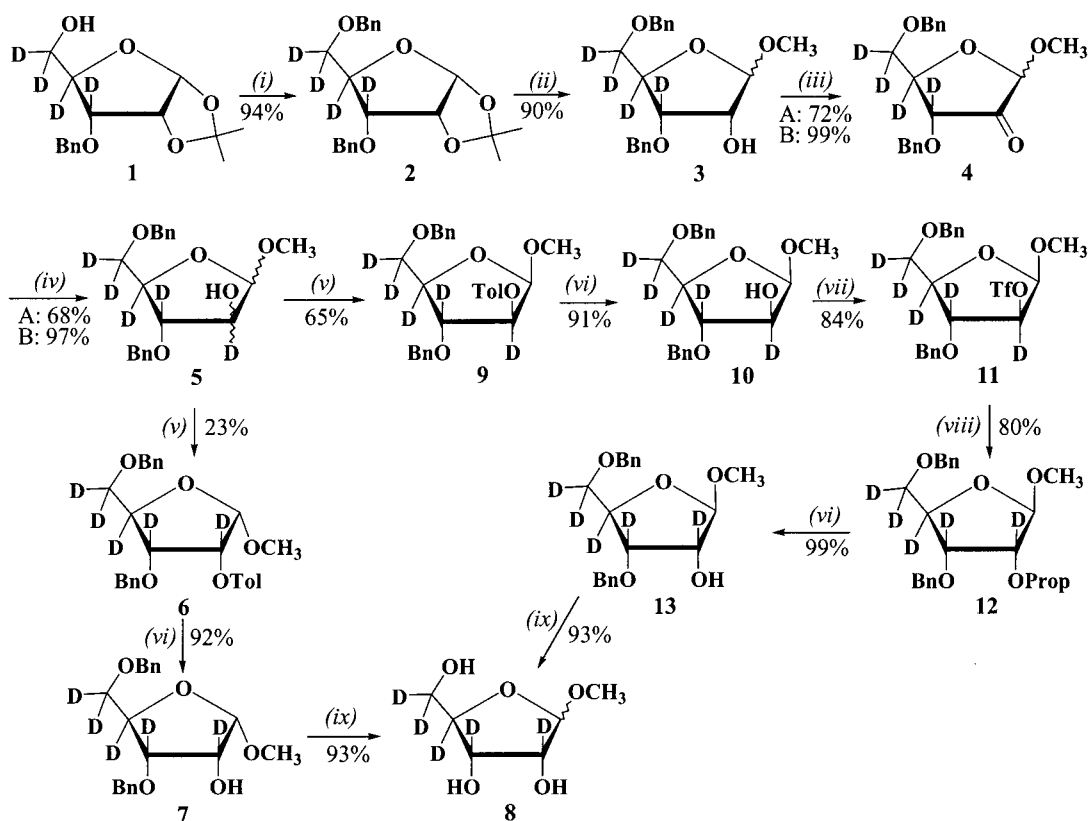
Scheme 1 a
