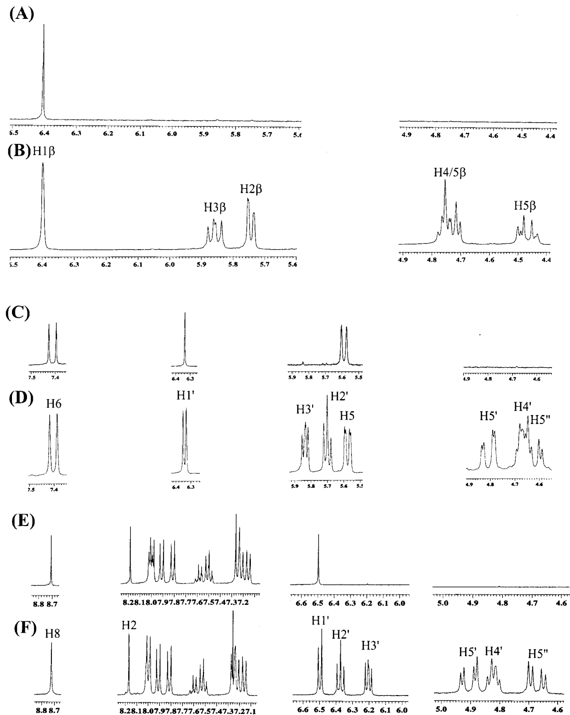
Figure 1. Expanded regions of the 270 MHz 1D 1 H NMR spectra of 1- O -acetyl-2,3,5-tri- O -(4-toluoyl)- \beta -D-ribose-2,3,4,5,5''- 2 H 5 ( 19 \beta ) (Panel A) and its natural abundance counterpart (Panel B), 2',3',5'-tri- O -(4-toluoyl)-uridine-2',3',4',5',5''- 2 H 5 ( 20a ) (Panel C) and its natural abundance counterpart (Panel D), 2',3',5'-tri- O -(4-toluoyl)- N 6 -benzoyladenine-2',3',4',5',5''- 2 H 5 ( 20b ) (Panel E) and its natural abundance counterpart (Panel F).
