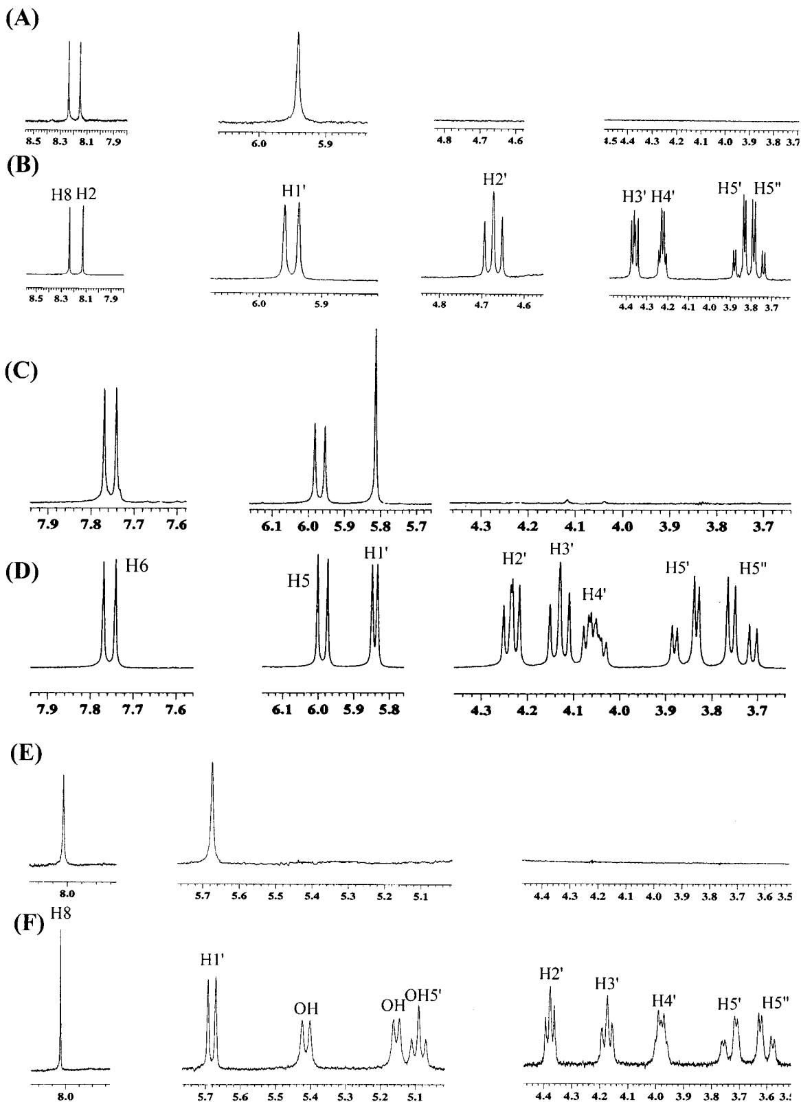
Figure 3. Expanded regions of the 270 MHz 1D 1 H NMR spectra of adenosine-2',3',4',5',5''- 2 H 5 ( 21b ) (Panel A) and its natural abundance counterpart (Panel B), cytidine-2',3',4',5',5''- 2 H 5 ( 21c ) (Panel C) and its natural abundance counterpart (Panel D), guanosine-2',3',4',5',5''- 2 H 5 ( 21d ) (Panel E) and its natural abundance counterpart (Panel F).
