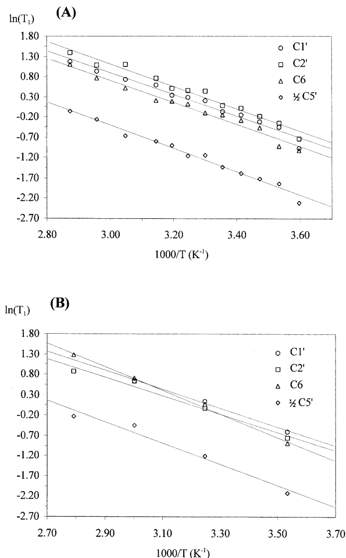
Figure 2. Longitudinal ^{13}\text{C} relaxation times as a function of reciprocal of temperature for (A) 2'-DT (1) and (B) anh-T (5b). For clarity only selected temperature-dependent T_1 values are shown for C-1' ( \circ ), C-2' ( \square ), C-6 ( \triangle ) and C-5' ( \diamond ) in both panels. Straight lines were obtained by linear regression and are characterized by the slope of -2.7 ( \sigma = 0.2 ) and intercept of 8.9 ( \sigma = 0.5 ) for C-1', the slope of -2.8 ( \sigma = 0.2 ) and intercept of 9.5 ( \sigma = 0.5 ) for C-2', the slope of -2.9 ( \sigma = 0.2 ) and intercept of 9.9 ( \sigma = 0.5 ) for C-3', the slope of -2.7 ( \sigma = 0.1 ) and intercept of 8.9 ( \sigma = 0.4 ) for C-4', the slope of -2.7 ( \sigma = 0.1 ) and intercept of 8.2 ( \sigma = 0.4 ) for C-5' in 2'-DT (1) and the slope of -2.3 ( \sigma = 0.2 ) and intercept of 7.6 ( \sigma = 0.5 ) for C-1', the slope of -2.3 ( \sigma = 0.2 ) and intercept of 7.3 ( \sigma = 0.8 ) for C-2', the slope of -2.9 ( \sigma = 0.1 ) and intercept of 9.7 ( \sigma = 0.1 ) for C-3', the slope of -2.2 ( \sigma = 0.3 ) and intercept of 7.2 ( \sigma = 0.8 ) for C-4', the slope of -2.9 ( \sigma = 0.1 ) and intercept of 9.4 ( \sigma = 0.4 ) for C-6' and the slope of -2.6 ( \sigma = 0.3 ) and intercept of 7.3 ( \sigma = 1.1 ) for C-5' in anh-T (5b).
