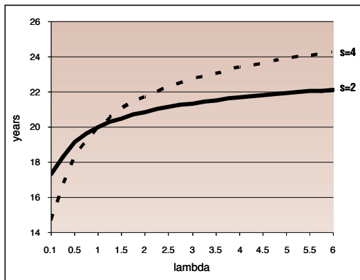
Figure 4. Optimal choice for e62
