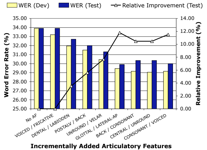
Fig. 5. Word error rates and relative improvements of incrementally added EMG articulatory feature classifiers in the stream architecture. The two AF sequences correspond to the best AF-insertion on the development subsets in two-fold cross-validation.
