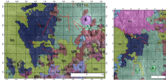
Fig. 1. Linear graben, crater chains and fissures (red lines) mapped in Sulpicius Gallus (left) and Rima Bode (right). Dark blue areas are mapped as pyroclastics on USGS maps [e.g., 15].
