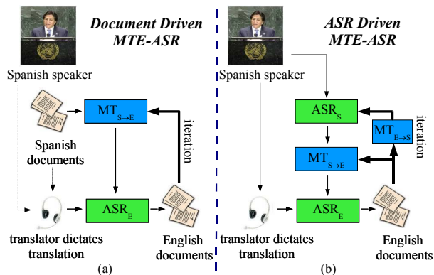
Figure 1: MT-Enhanced ASR
