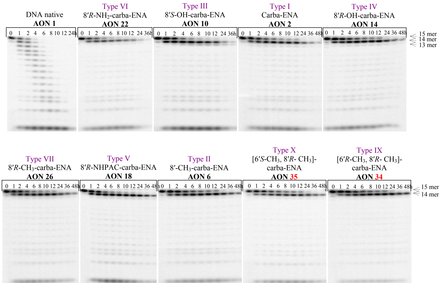
FIGURE SII 15. Autoradiograph of 20% denaturing PAGE showing the stability of 5'- 32 P-labeled AONs in human serum.
