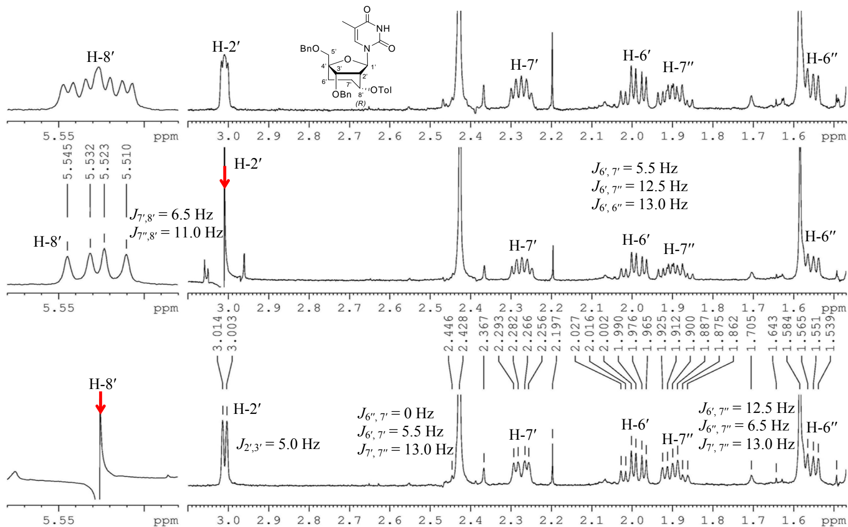
Figure SII. 12. Homodecoupling spectrum of compound 21b
