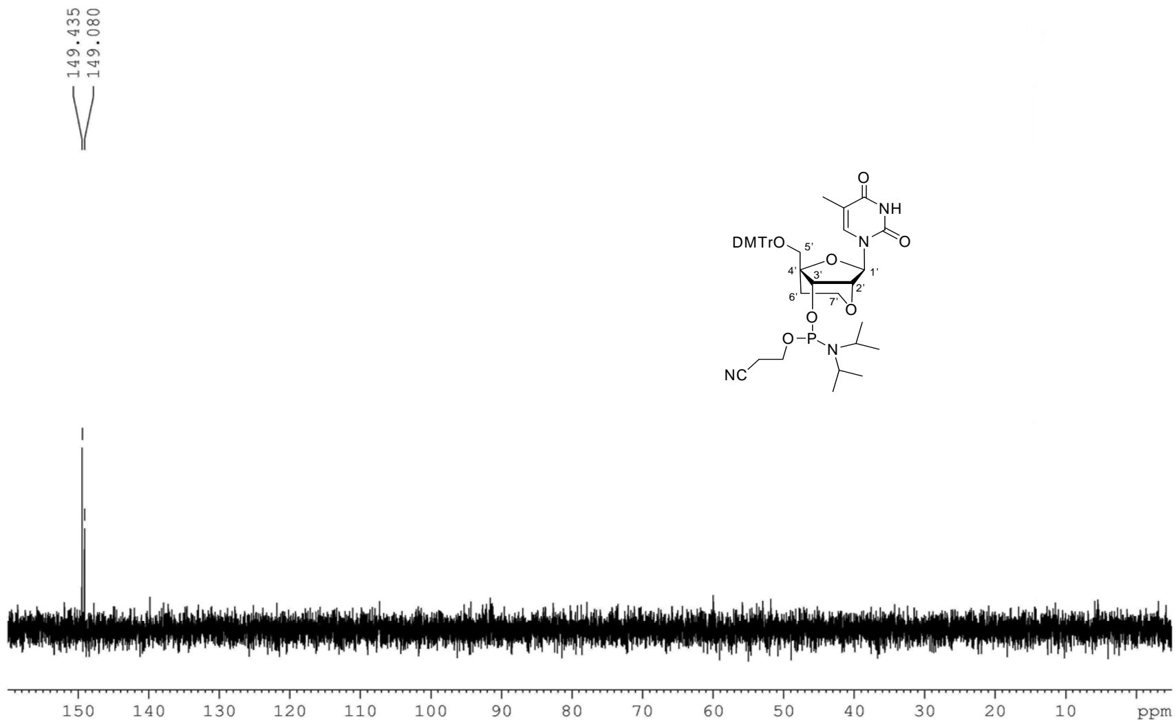
Figure SII. 22. ^{31}\text{P} NMR spectrum of compound 37
