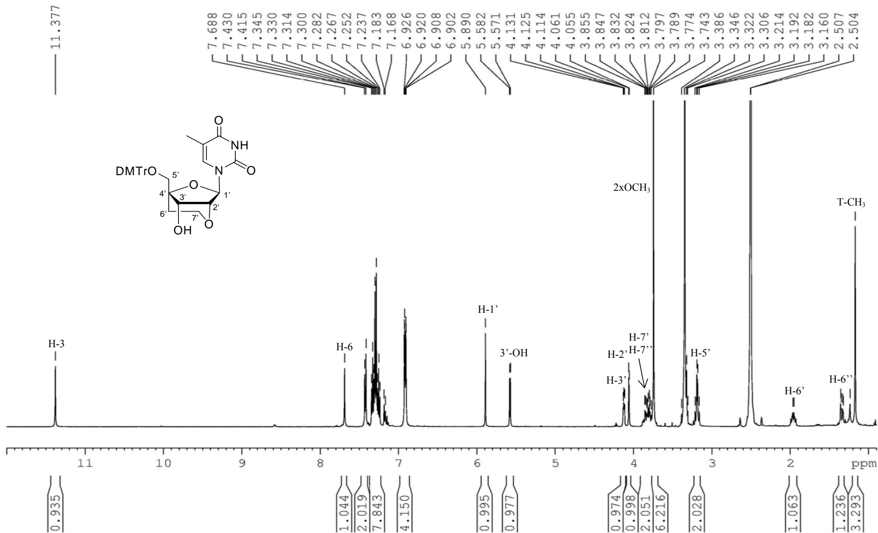
Figure SII. 21. 1 H NMR spectrum of compound 36
