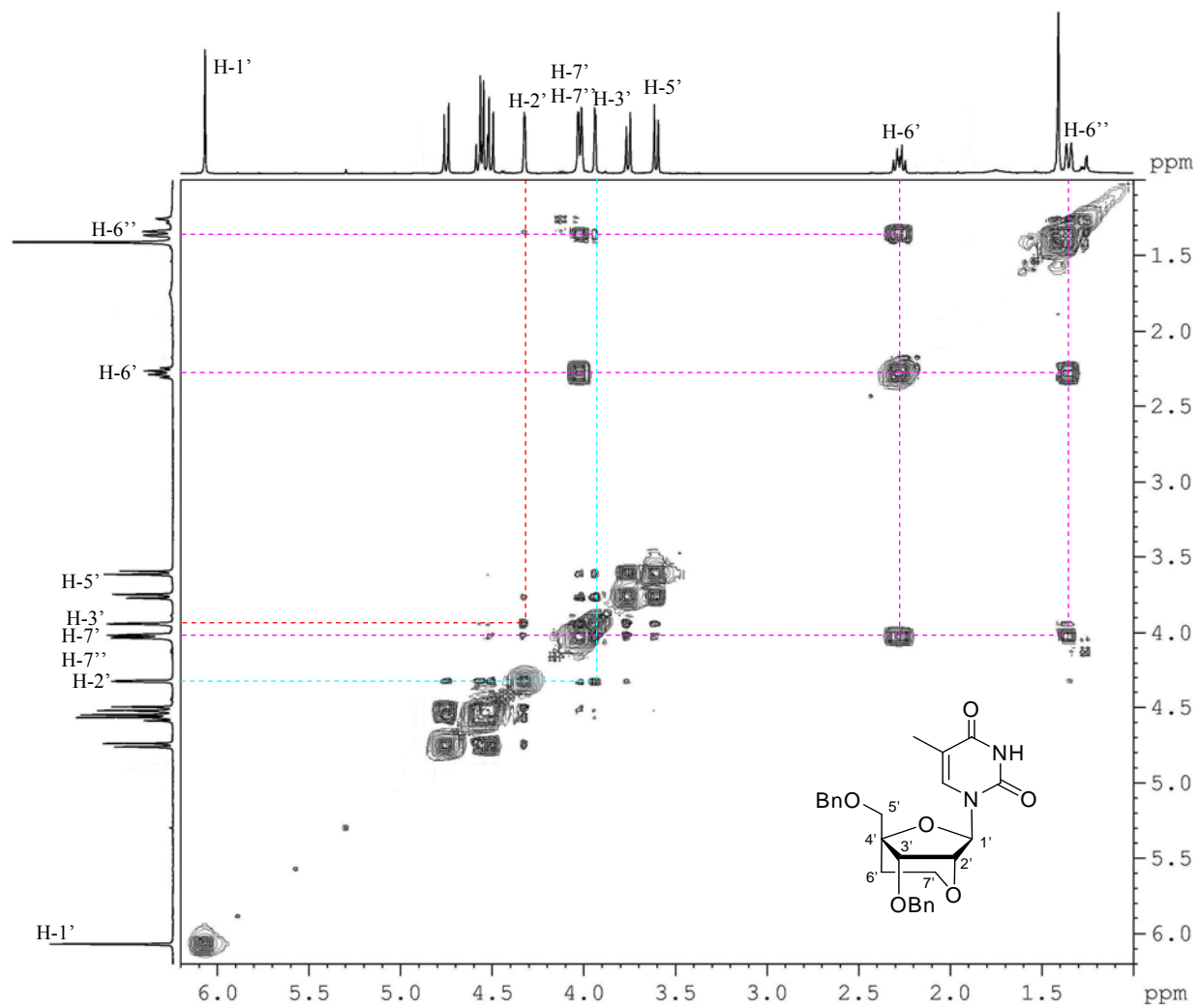
Figure SII. 18. Expansion of COSY spectrum of compound 34
