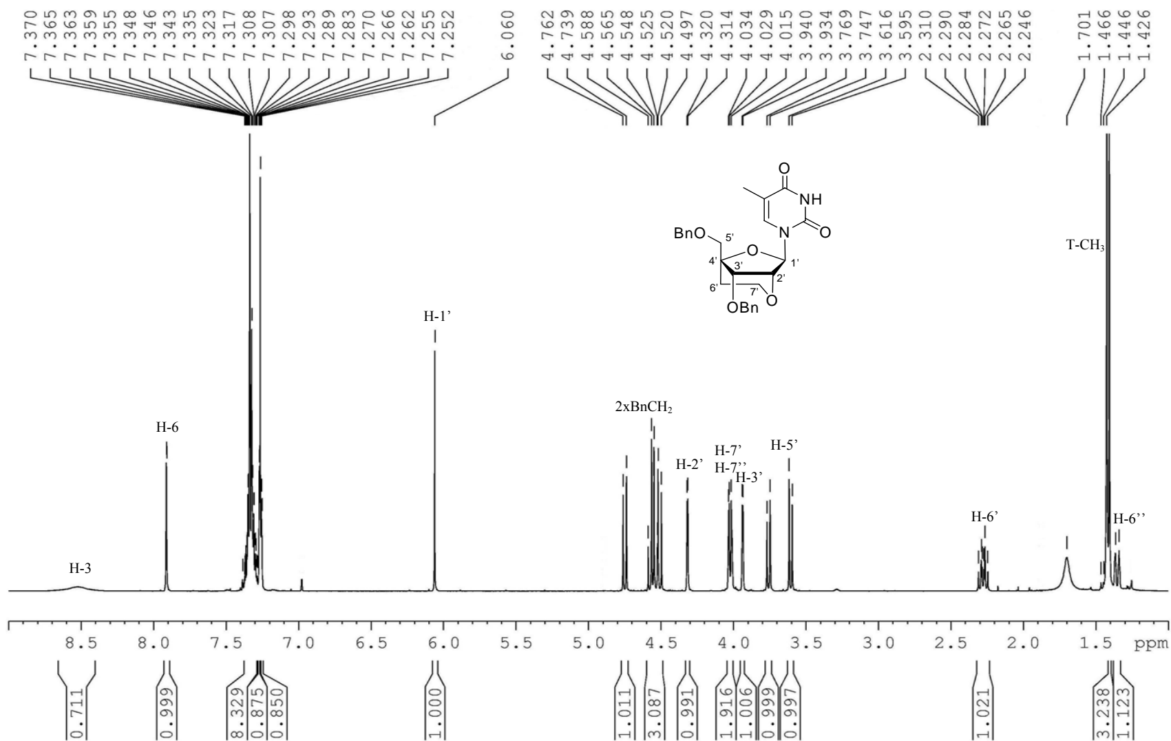
Figure SII. 16. ^1\text{H} NMR spectrum of compound 34
