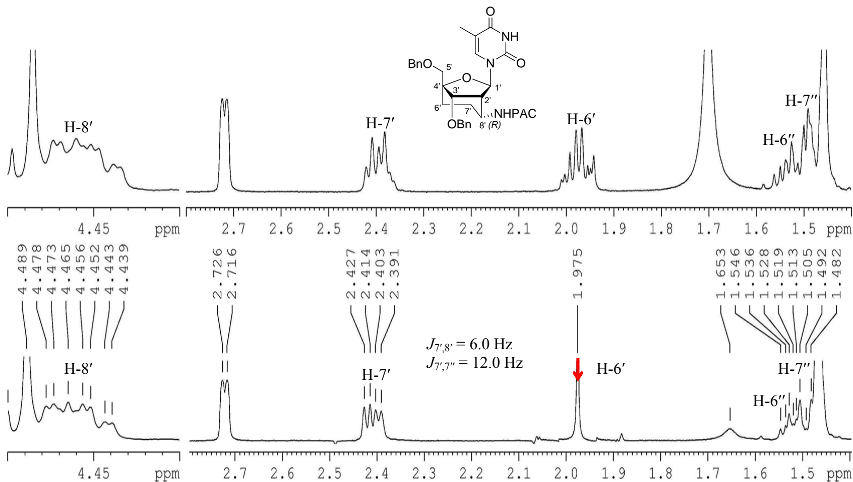
Figure SII. 9. Homodecoupling spectrum of compound 16b (H6' decoupled)
