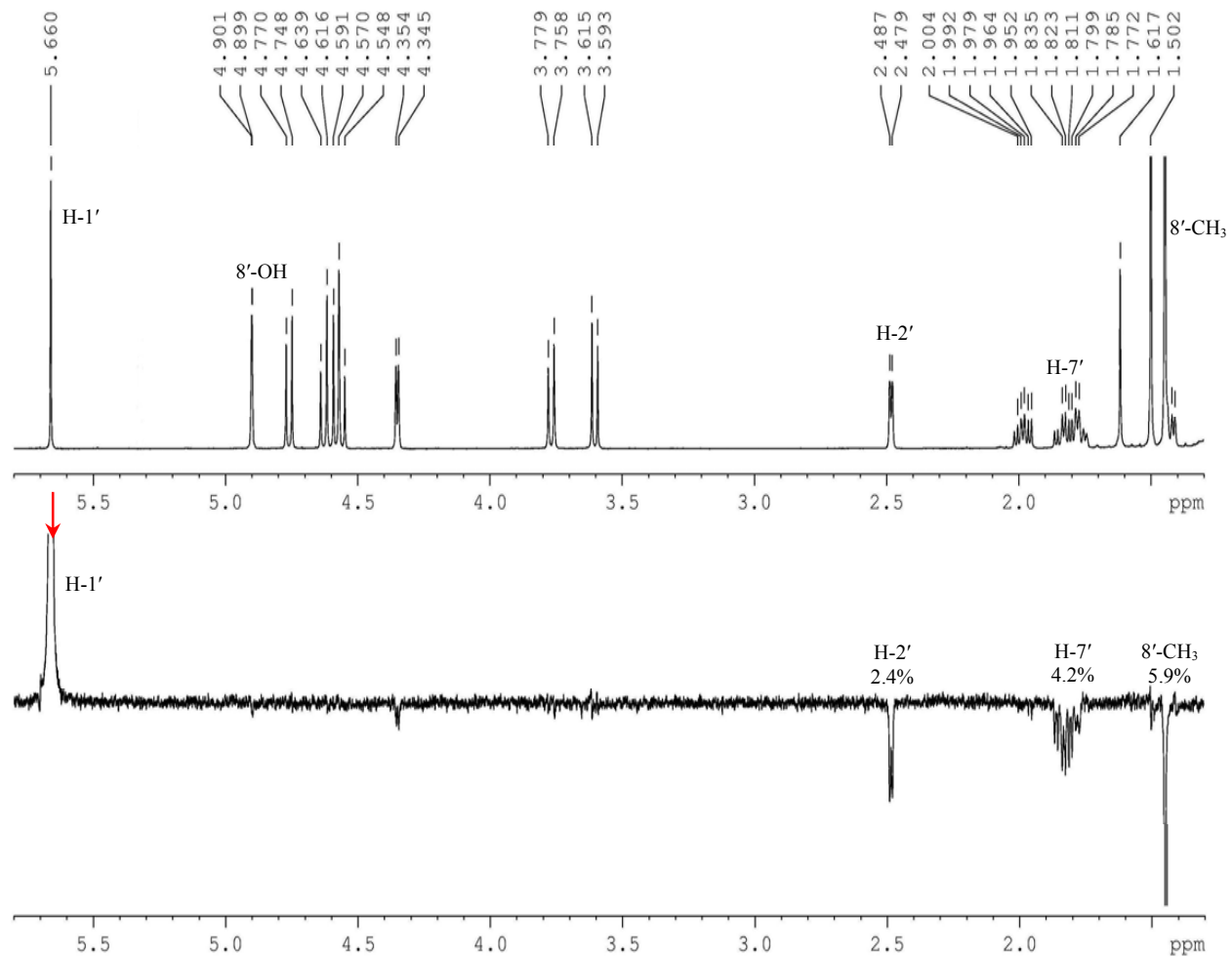
Figure SII. 4. 1D nOe spectrum of compound 26 (H1' irradiated)
