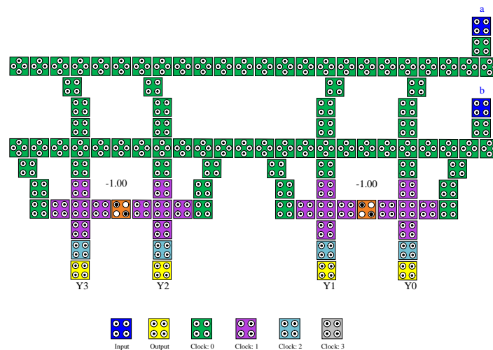
Fig.1. proposed combinational circuit using inverter chains
