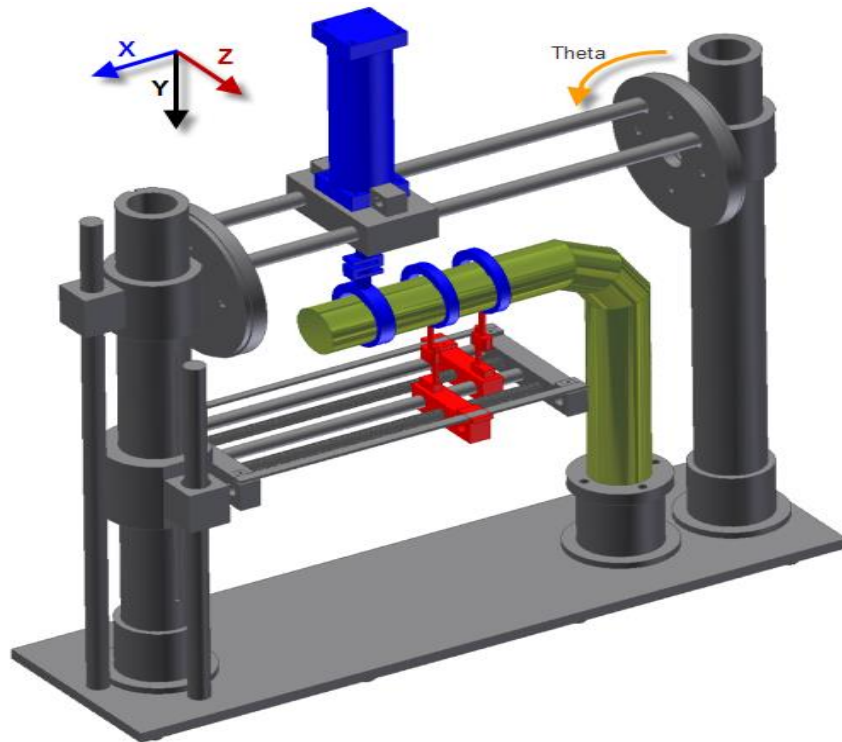
Figure 2. Three Dimensions Model for Special Testing Machine (STM)
