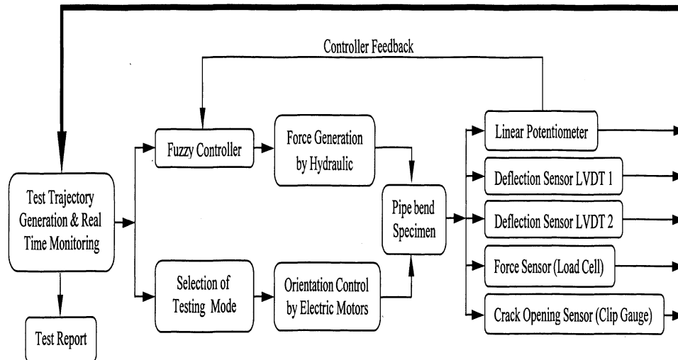
Figure 3. Block Diagram for Control Loop and Signal Monitoring Loop
