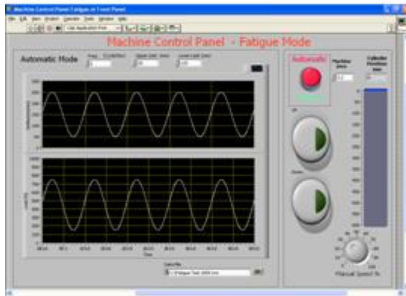
Figure 5. Front Panel for the Control System
