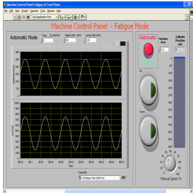
Front Panel for the Control System
