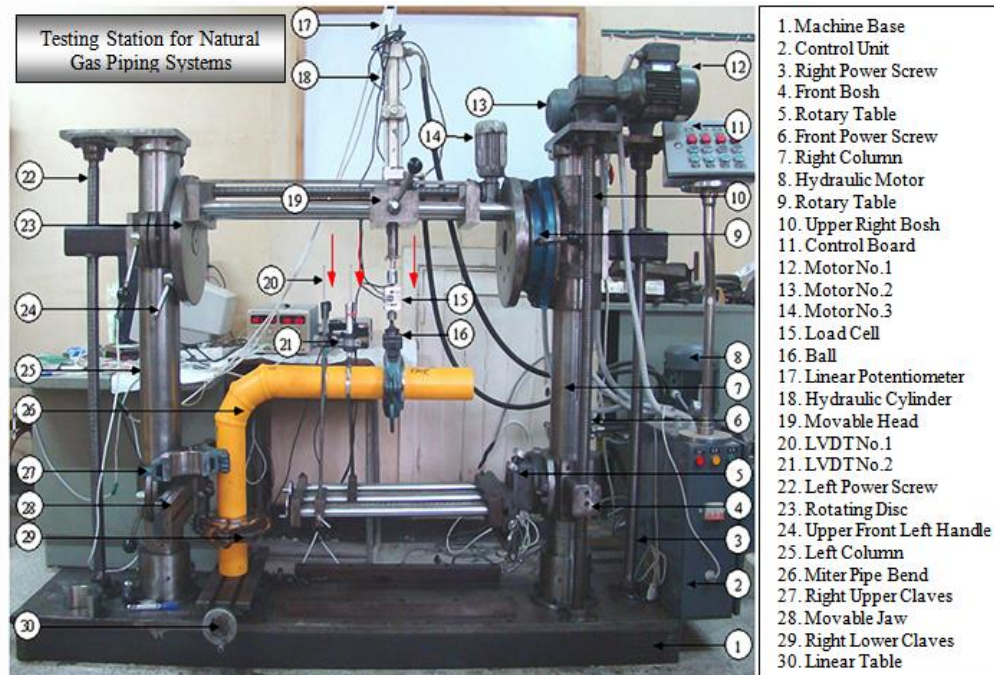
Figure 1. Photo of Testing Machine for Natural Gas Piping Systems (NGPS)
