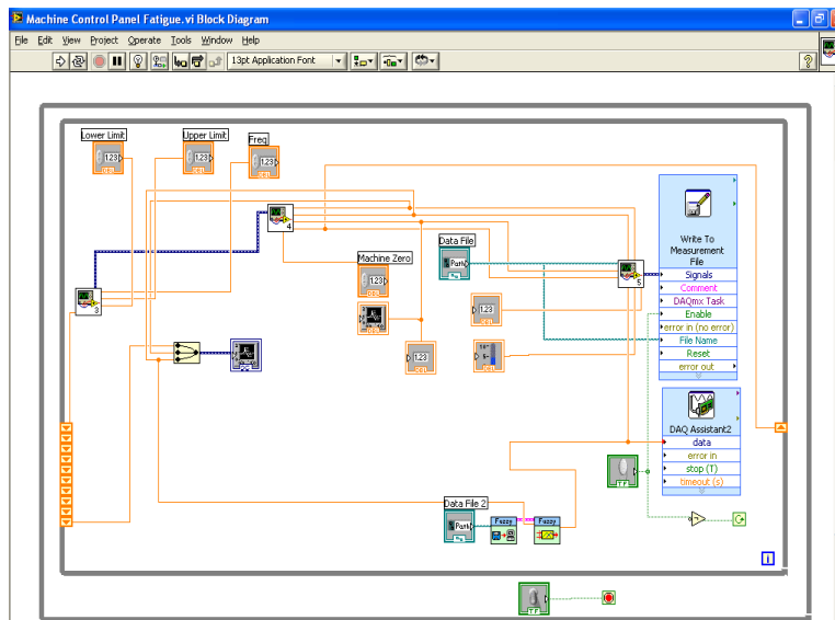
Block Diagram for the Control System
