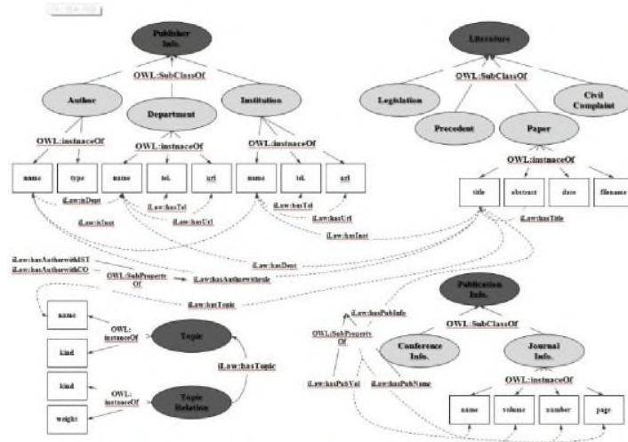
Fig. 2 Semantic Data Model in Suggested Service
