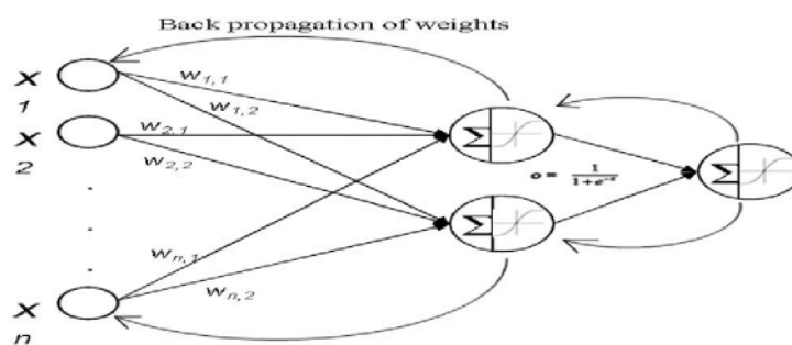
Fig. 1. Typical architecture of Back propagation Neural Network
