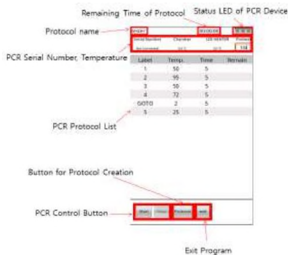
Fig. 1 Android Smartphone Main UI
