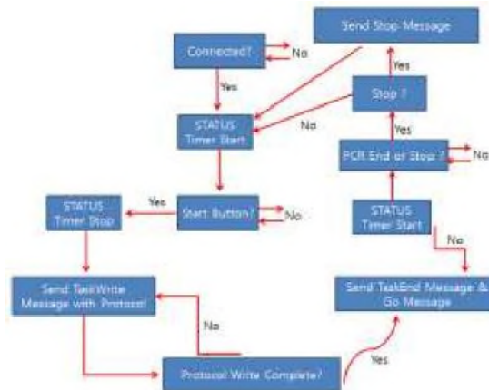
Fig. 2 Flow chart of the PCR control program
