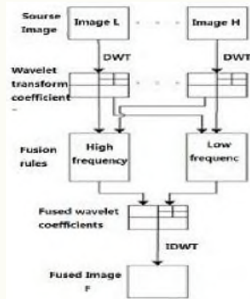
Fig. 1 Processes of image fusion algorithm
