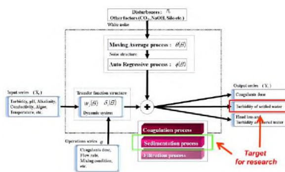
Fig. 1. Schematic diagram of TF-ARIMA model for sedimentation process
