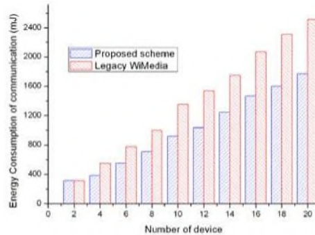
Fig. 4. Communication energy consumption of the WiMedia network with different scales
