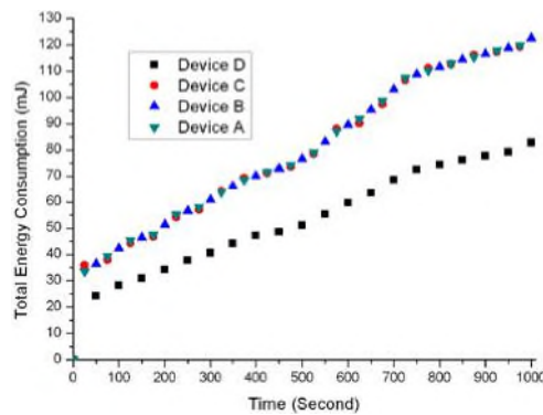
Fig. 3. Energy consumption of device according to the operating time of WiMedia device
