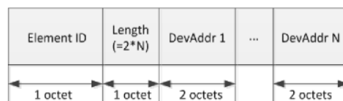
Fig. 2. The format of TIM IE
