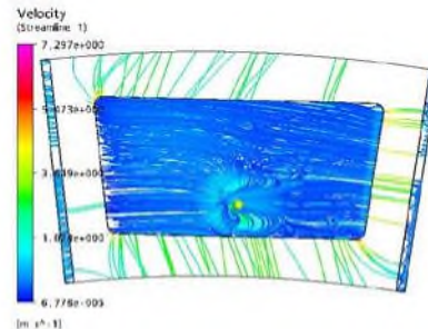
Fig.3. Streamlines of 36L/min inlet flow
