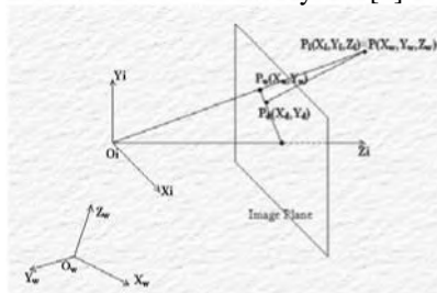
Fig. 3. Tasi camera calibration algorithm Camera calibration
