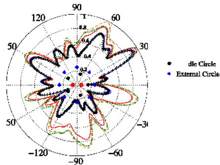
(a) The desired signal arrives (\theta, \phi) = (90, 30) and one interfered signal arrives from (\theta, \phi) = (90, -30)
