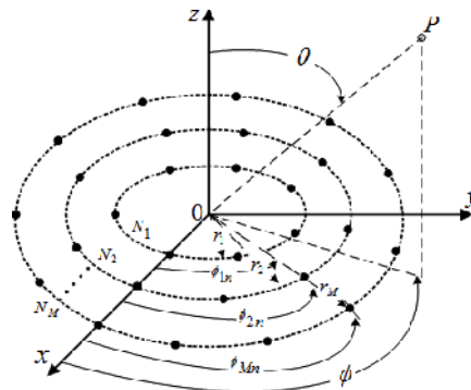
Fig. 2. Concentric circular arrays (CCAA)
