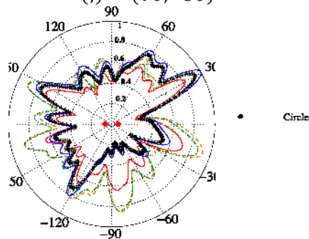
(b) The desired signal arrives (\theta, \phi) = (90, 30) and two interfered signals arrive from (1, 1) = (90, -30) and (2, 2) = (90, -60)
