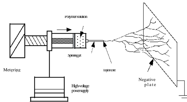
Figure 1 Electrospinning Device
