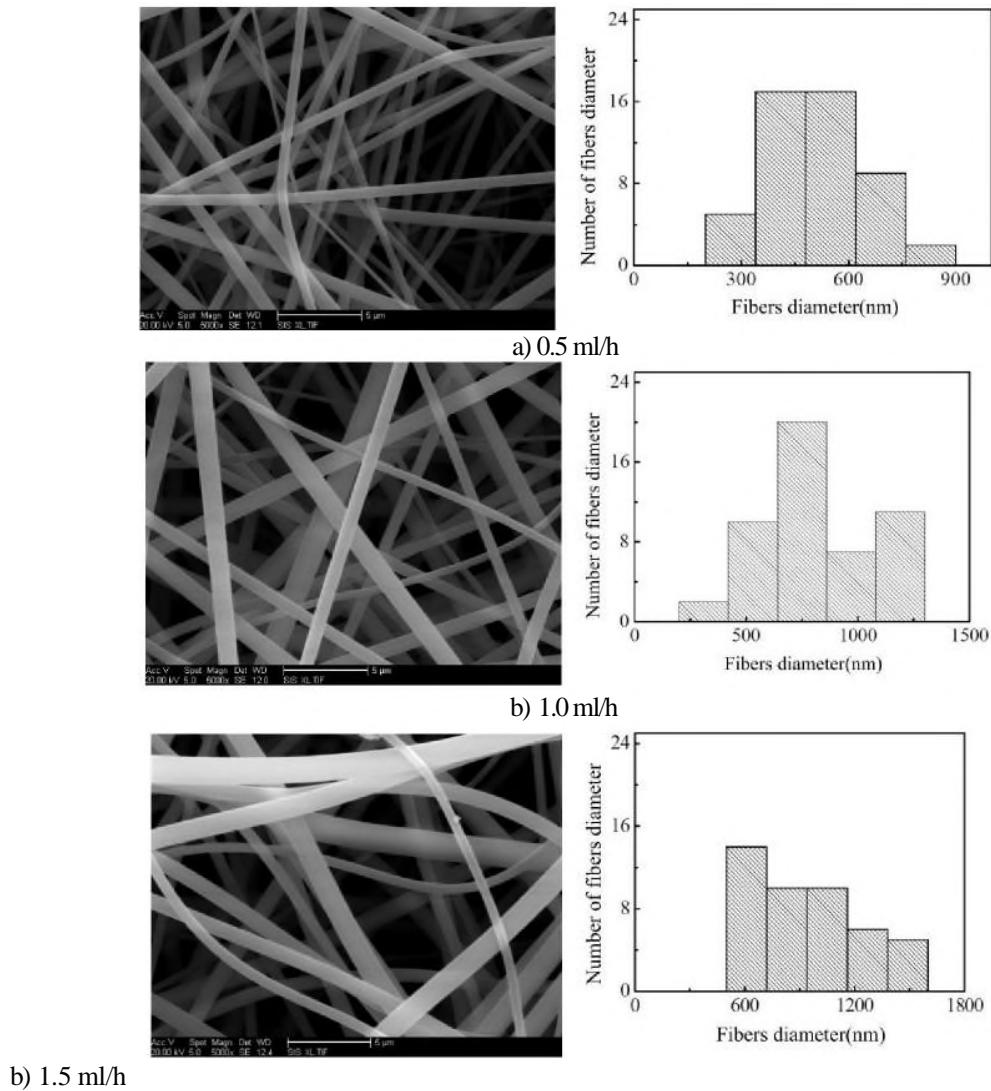
Figure 9. Polyimide Nanofibers SEM Images and Fibers Diameter Distribution Histogram with Different Extrusion Speed
