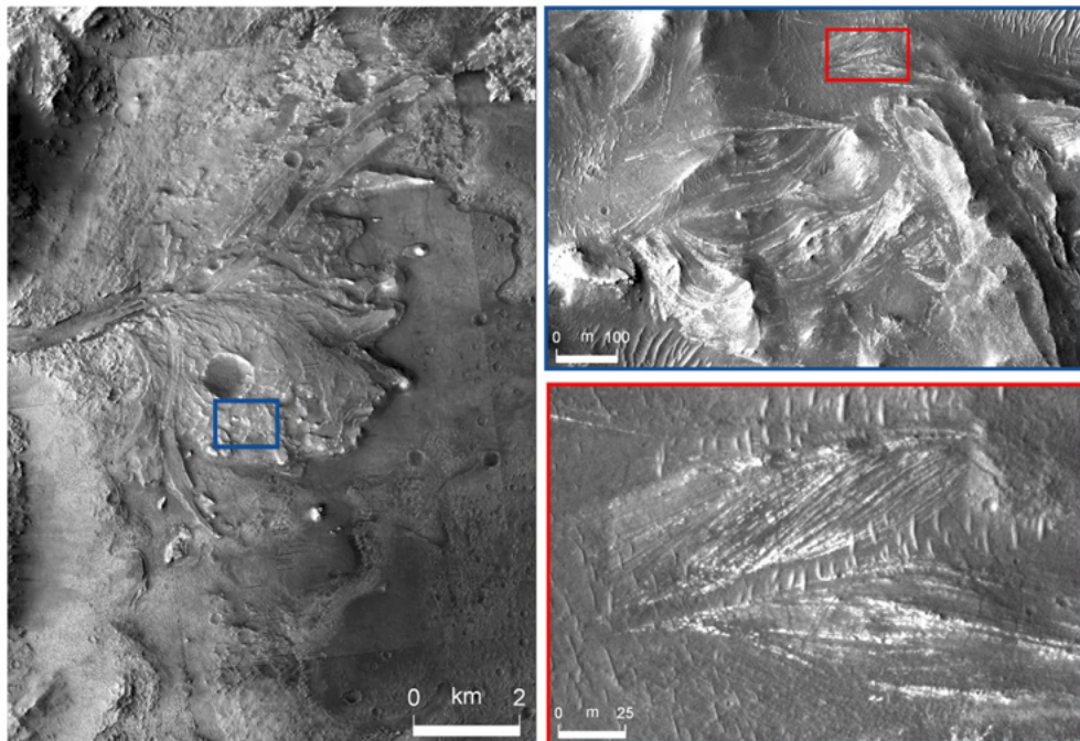
Figure 5. Topography of Jezero Crater.
