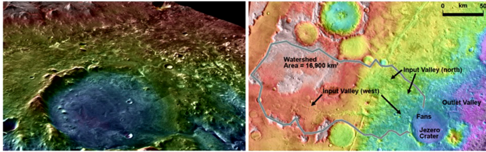
Figure 4. Jezero Crater in perspective view showing Isidis Basin rim and watershed area.
