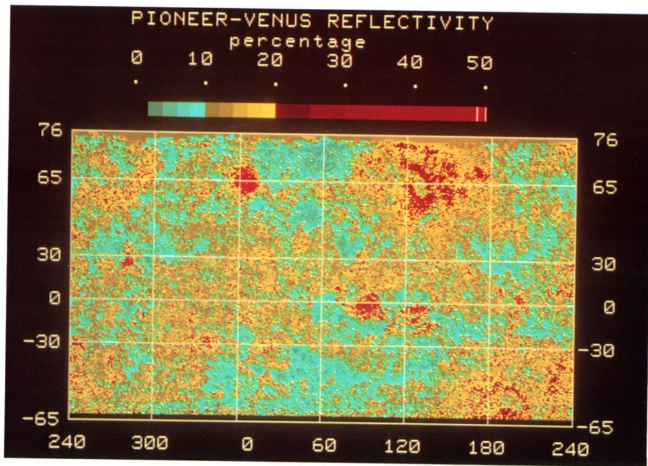
Plate 3. Mercator map of reflectivity with three subdivisions corresponding to soil-dominated (blue), rock-dominated (yellow), and high dielectric dominated surfaces (red).
