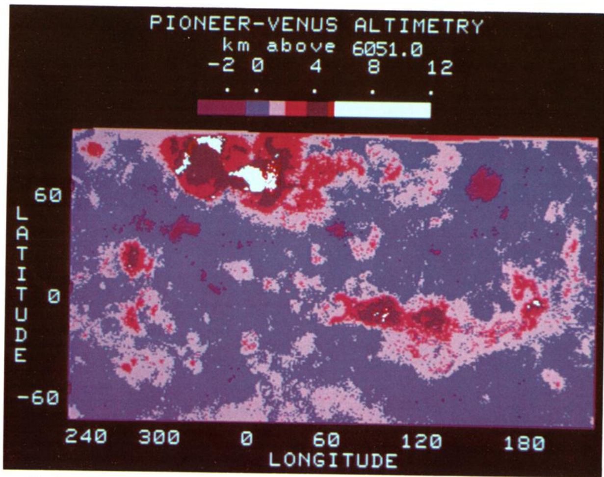
Plate 2. Mercator map ( 1^\circ \times 1^\circ ) of topography in which zones are identified by color (e.g., pink is zone IV from Figure 4). Note that zones I and II and VII and VIII have been combined for display purposes.
