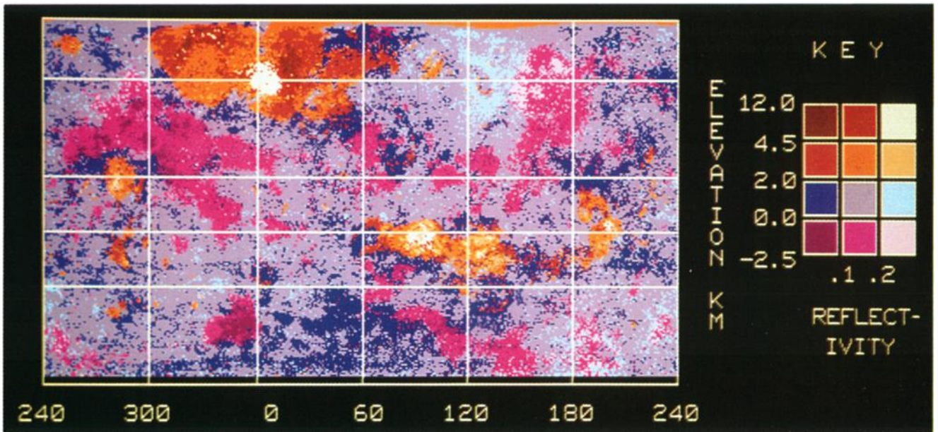
Plate 6. Map of elevation versus reflectivity. Twelve subdivisions are defined on the basis of the divisions of elevation and reflectivity shown in Plates 2 and 4 and discussed in the text. Hue is used to show divisions in elevation, and intensity to show divisions in reflectivity.
