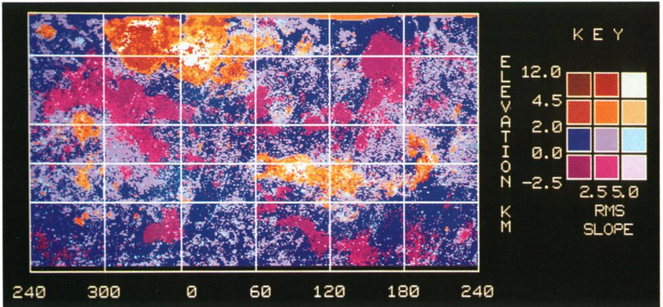
Plate 5. Map of elevation versus roughness. Twelve subdivisions are defined on the basis of the divisions of elevation and roughness shown in Plates 2 and 3 and discussed in the text. Hue is used to show divisions in elevation and intensity to show divisions in roughness.
