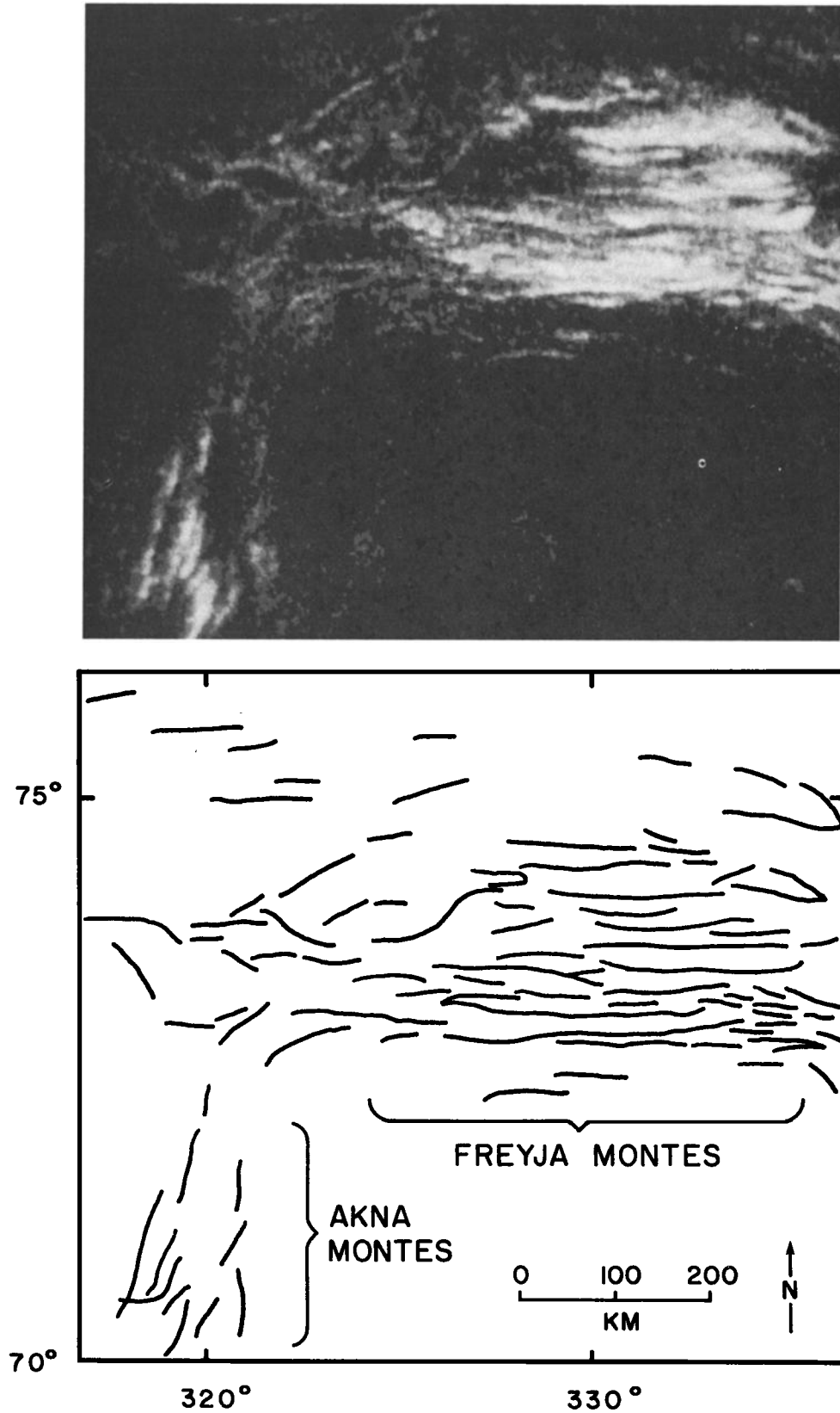
Fig. 1. (Top) Radar image of banded terrain in Ishtar Terra obtained at 12.6-cm wavelength by the Arecibo Observatory [Campbell et al. , 1983]. Bright areas are relatively rougher than dark areas at centimeter to decameter scales. (Bottom) Sketch map of the same area, outlining linear bands of high radar backscatter in Freyja Montes and northern Akna Montes.
