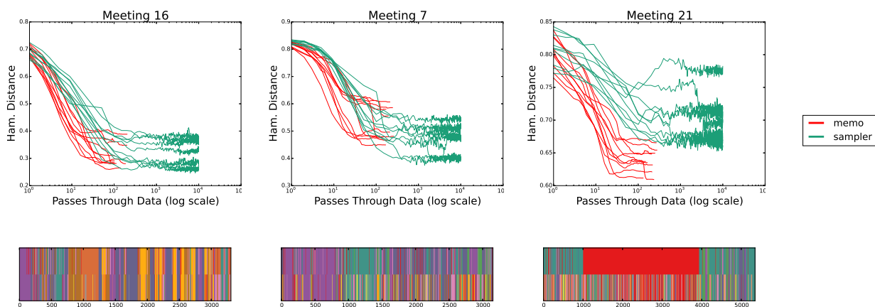
Figure 8: Speaker Diarization results. Top : Plots of hamming distance vs. pass through data for meetings 16, 7, and 21, representing best, intermediate and worst performance, respectively. Bottom : Comparison of estimated state sequence labels (bottom half of each image) with true labels (top half of each image).
