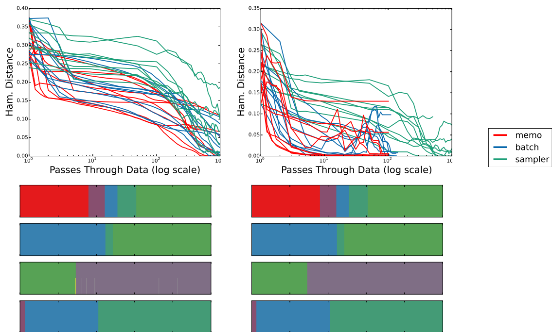
Figure 7: HMM toy dataset results. Top : Plot of hamming distance versus pass through data for the sampler and our single batch and memoized algorithms with \kappa = 0 (left) and \kappa = 100 (right). Bottom : Comparison of estimated state sequence labels (bottom half of each image) with true labels (top half of each image). Shown are four of the thirty-two estimated sequences from the best run of our memoized algorithm.
